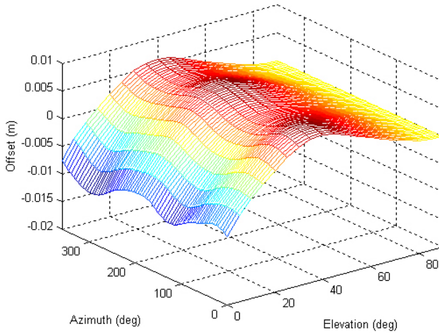
Leica choke L1 phase center offsets
