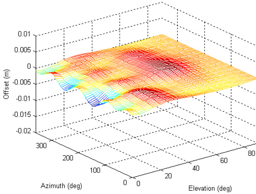
Zephyr L1 phase center offsets
