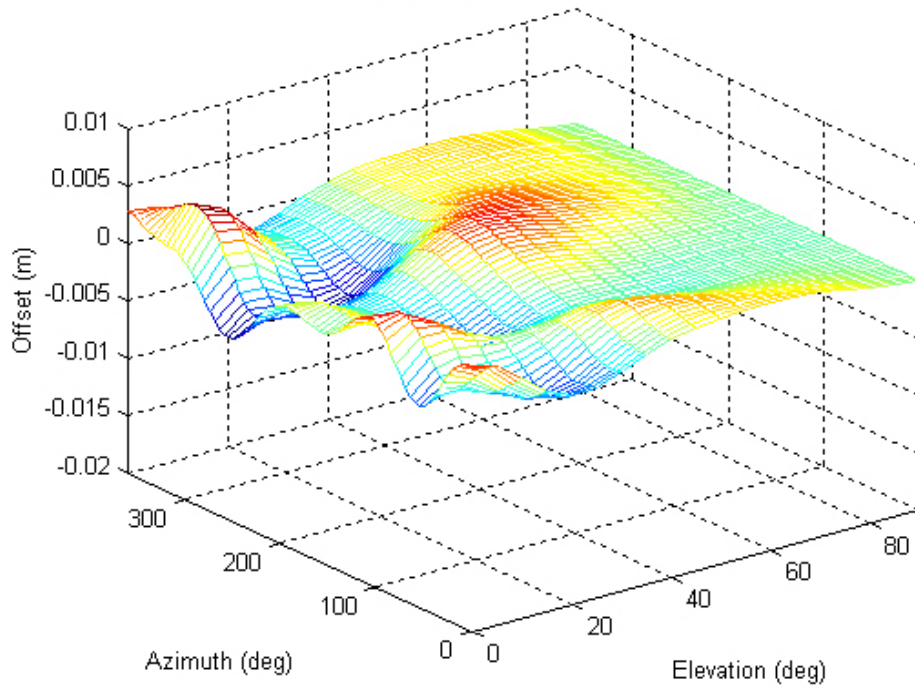
Zephyr L2 phase center offsets
