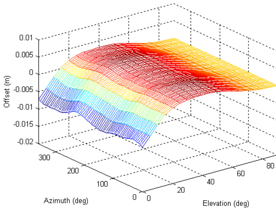
Leica Choke L2 phase center offsets
